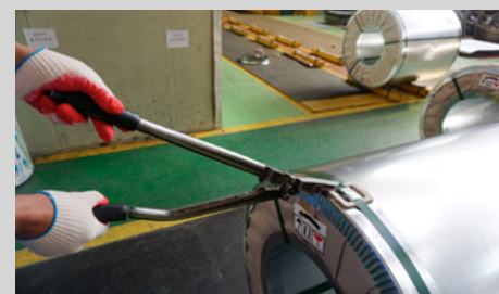
▲ Cut from the side of coil when cutting band
