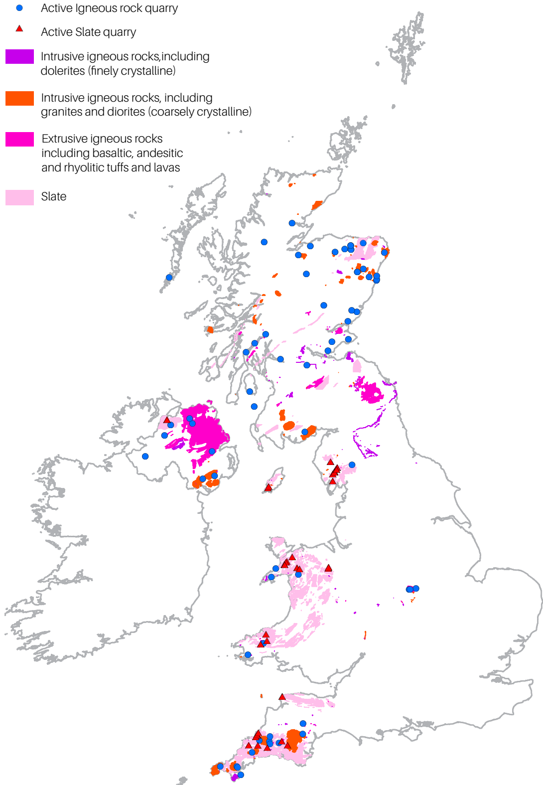
Figure 3 Distribution of principal igneous rock and slate resources and active quarries. Includes stone used for paving, roofing and hard landscaping.
