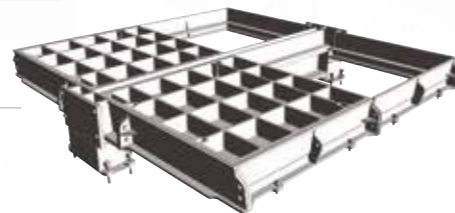
Type RRF recessed
