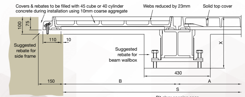
Section D - D
