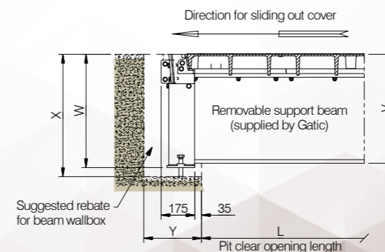
Solid top cover - Type RSF
