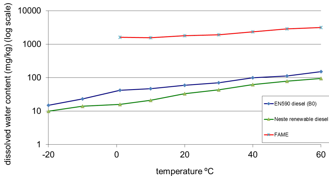
Figure 7. Water absorption properties of EN 590 diesel, Neste Renewable Diesel and FAME were demonstrated with laboratory experiments under a wide temperature range and excess amount of supplemented water.
