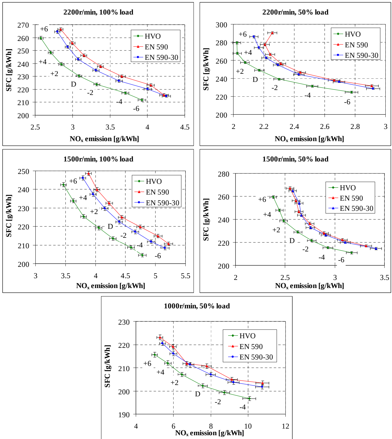
Figure 6. Trade-off between \text{NO}_x and specific fuel consumption (SFC). "D" means the default main injection timing. + or - sign and the number means a start of main injection in ^\circ\text{CA} after or before the default setting.
