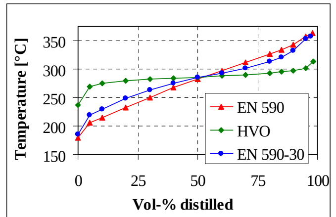
Figure 3. Distillation curves of the test fuels.
