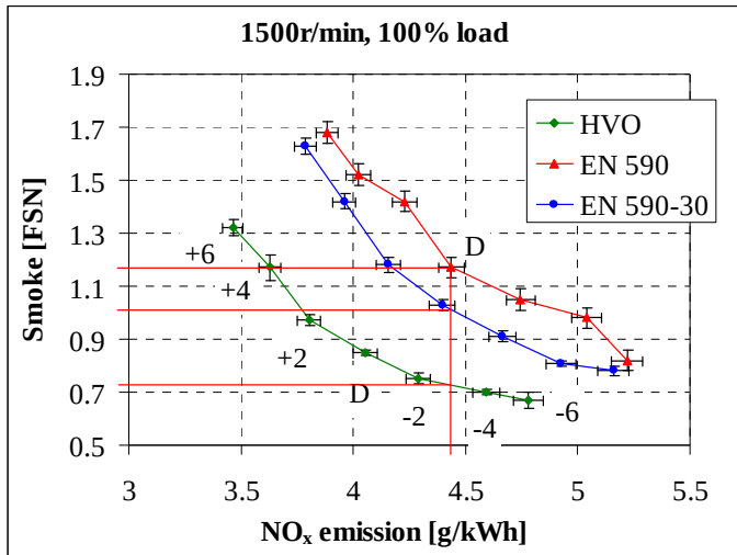
Figure 7. Example how smoke is obtained when \text{NO}_x is considered equal between the test fuels.
