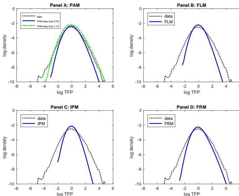
Figure 6: TFP Distribution
